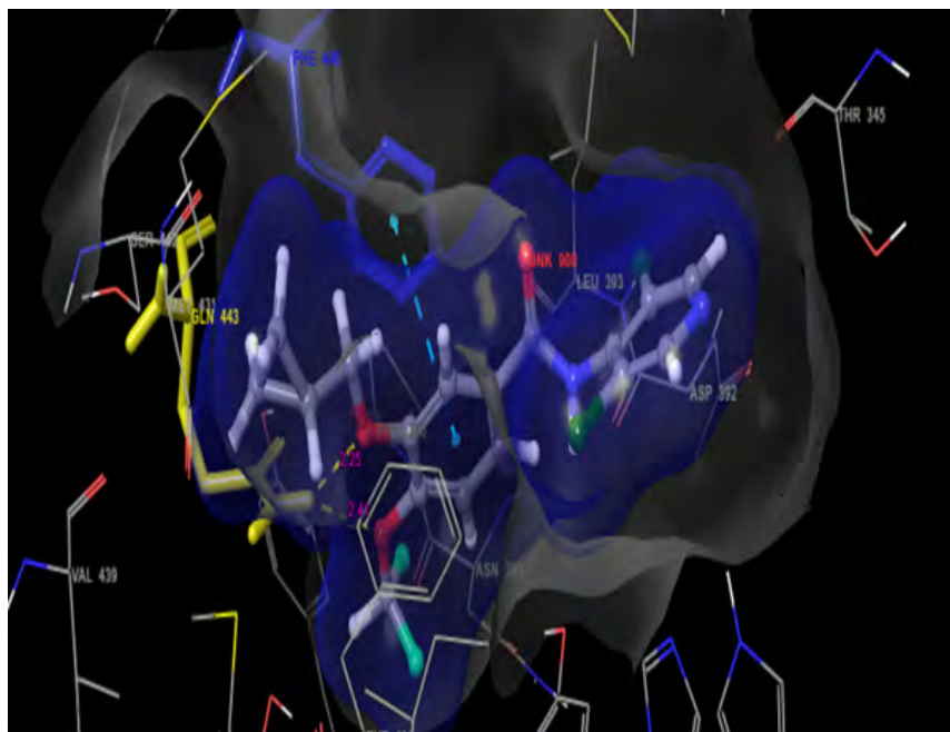
Figure 1a: Visualization of 1XMU protein using Maestro.
